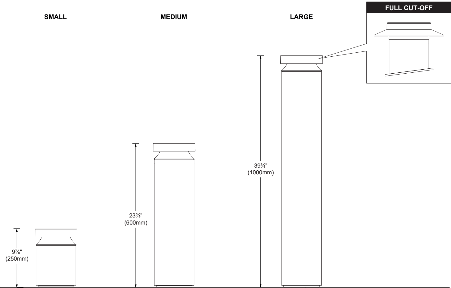
SIDE VIEW
