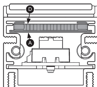
HONEYCOMB
