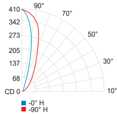
BO WGM + microlouver (3000K, 80CRI)
