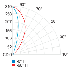
BO WGWF + microlouver (3000K, 80CRI)
