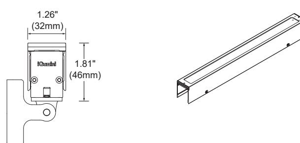
A8- Protective frame (For IK10)
