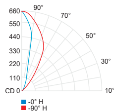
BO elliptical (3000K, 80CRI)
