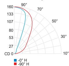
BO General light no-dot (3000K, 80CRI)
