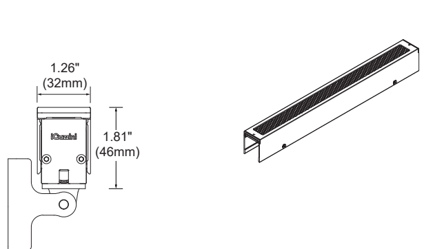
A5- Honeycomb louver
