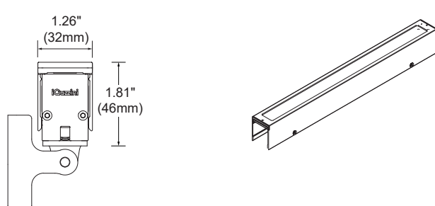
A7- Linear prismatic screen
