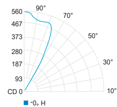
BO Wide flood (3000K, 80CRI)
