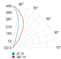
BO WGWF (3000K, 80CRI)
