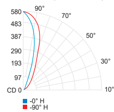
BO WGM (3000K, 80CRI)
