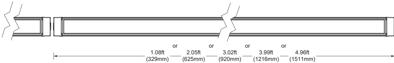
TOP VIEW
