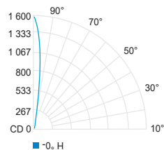
BO WGS + microlouver (3000K, 80CRI)
