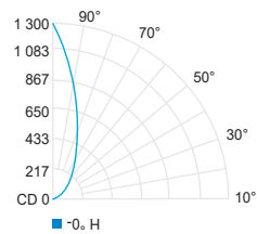
BO Flood (3000K, 80CRI)
