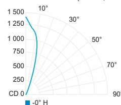
Flood 30° BO (3000K, 80CRI)
