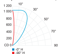
Elliptical 78° / 10° BO (3000K, 80CRI)
