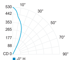
Wide flood comfort 42° BO (3000K, 80CRI)
