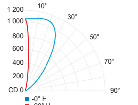
Elliptical 78° / 10° BO (3000K, 80CRI)
