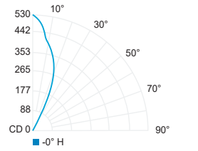
Wide flood comfort 42° BO (3000K, 80CRI)
